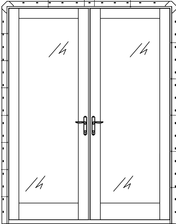
EXTERIOR ELEVATION
